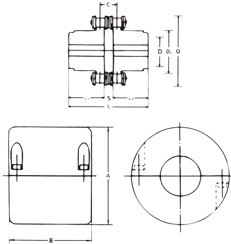
Casing
